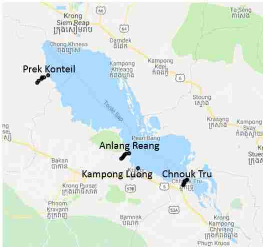
Figure 4.1. Map of the in-situ data observation locations. Prek Kunteil, Anland Reang and Chnouk Tru all include 6 observation locations (Miller, 2015). Kampong Luong only has one location (MRC, 2011)
