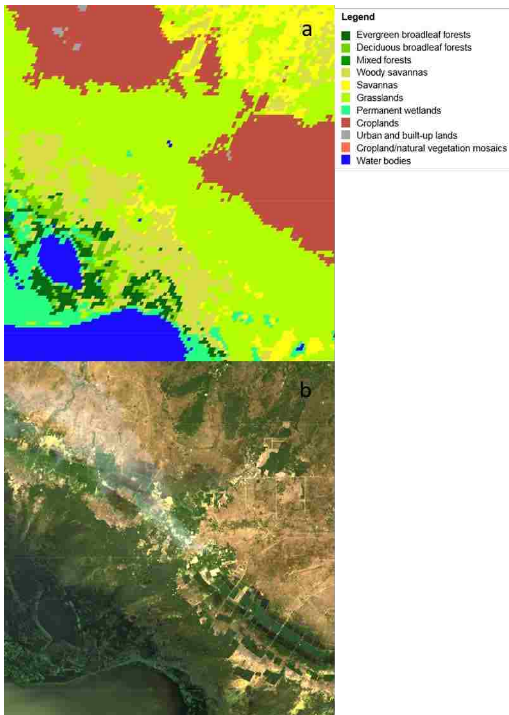
Figure 3.7. a) Map of the IGBP land cover classification in Tonle Sap floodplain and b)
